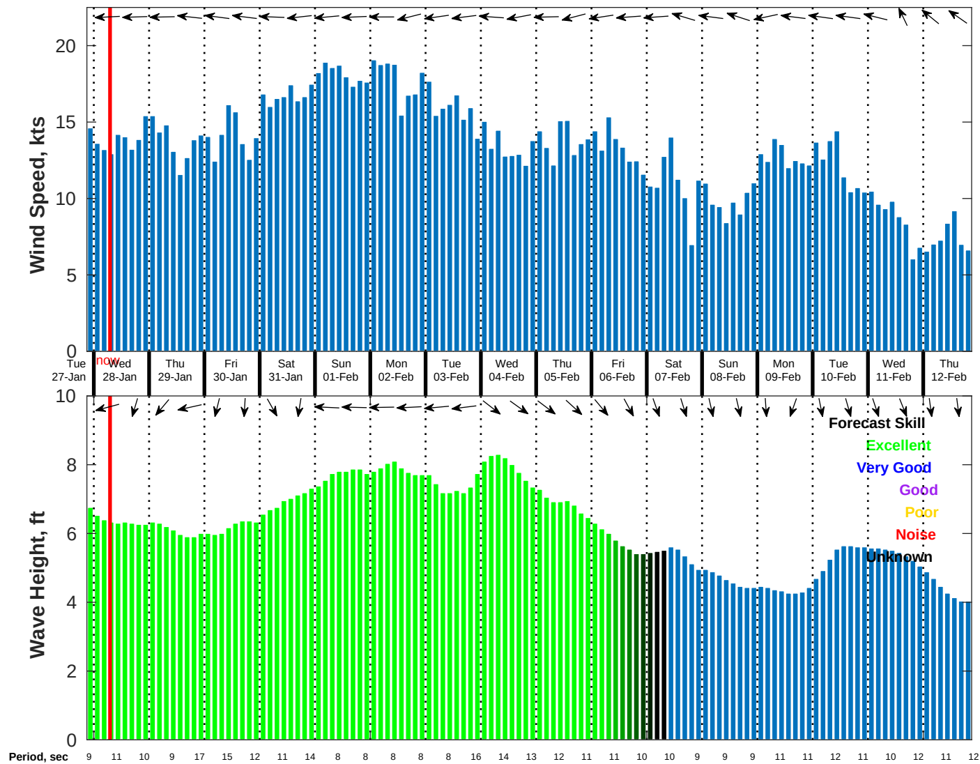
Wind & Wave Forecast for NDBC 41040 from 27-Jan-2026 21:00:00 to 12-Feb-2026 21:00:00
