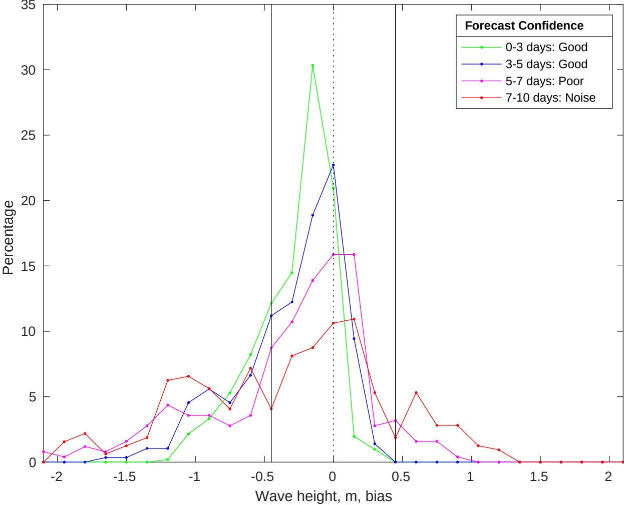
NDBC 42019 vs CMEMS Waves Bias Histogram: 28-Jan-2026
