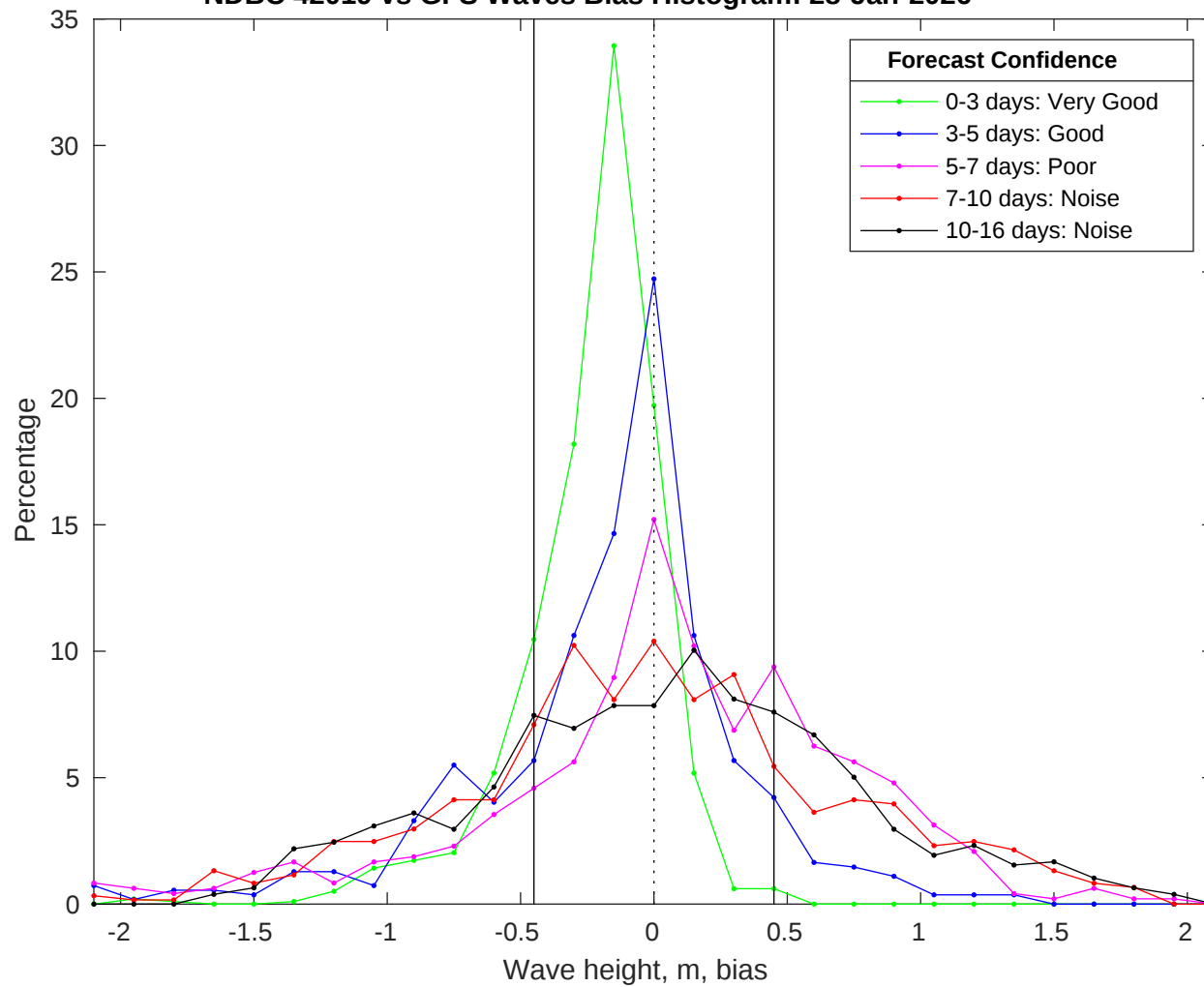
NDBC 42019 vs GFS Waves Bias Histogram: 28-Jan-2026
