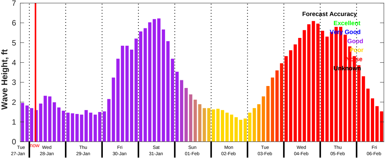
CMEMS Wave Forecast for NDBC 42019 from 27-Jan-2026 18:00:00 to 06-Feb-2026 18:00:00
