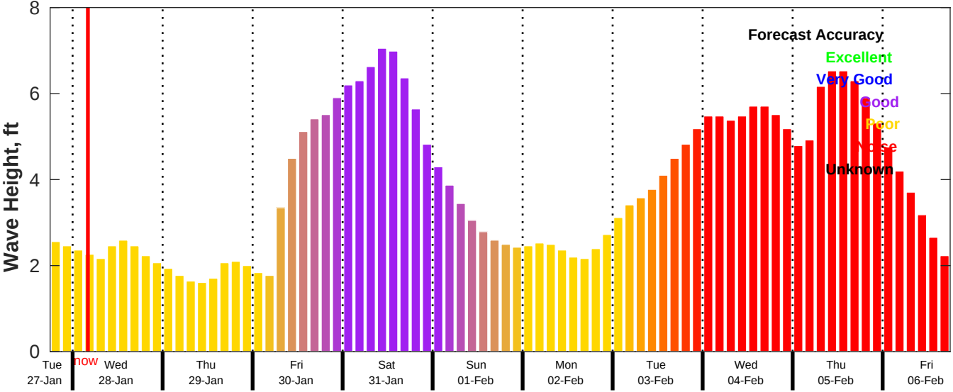
CMEMS Wave Forecast for NDBC 42020 from 27-Jan-2026 18:00:00 to 06-Feb-2026 18:00:00
