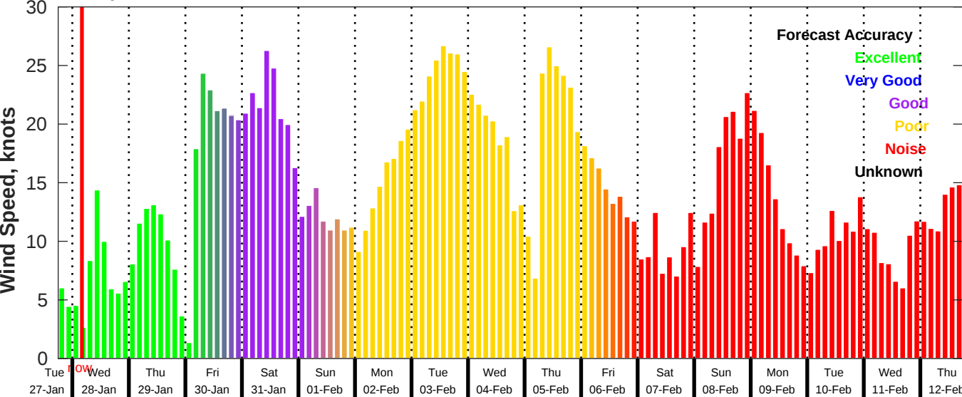
GFS Wind Speed Forecast for NDBC 42020 from 27-Jan-2026 18:00:00 to 12-Feb-2026 18:00:00
