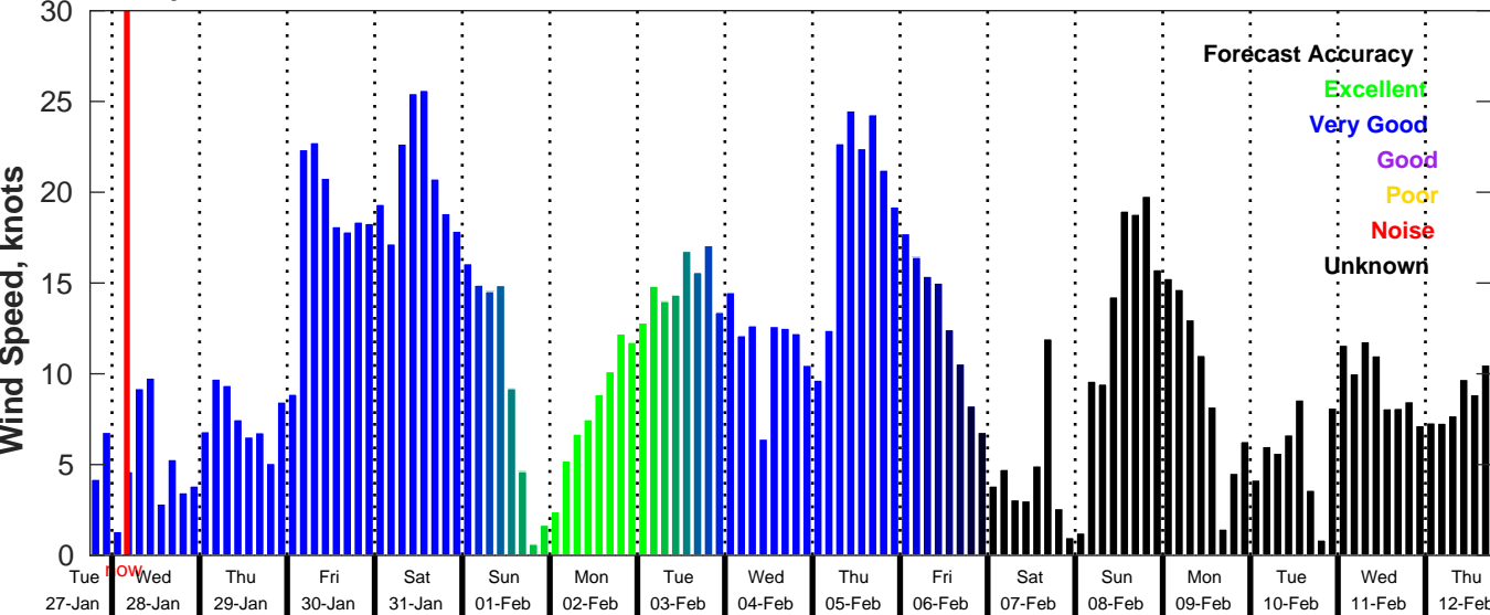
GFS Wind Speed Forecast for NDBC 42035 from 27-Jan-2026 18:00:00 to 12-Feb-2026 18:00:00
