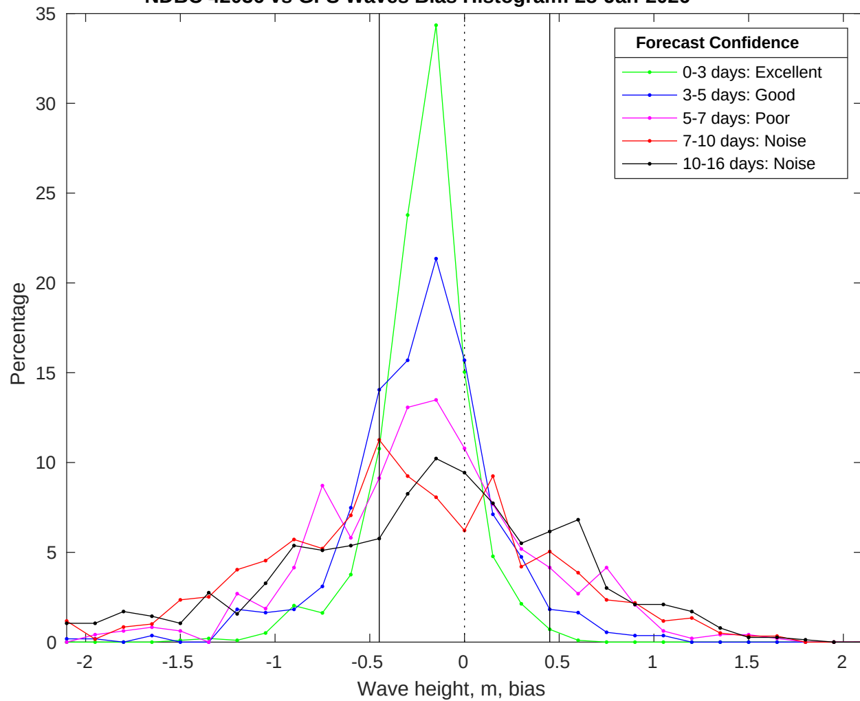
NDBC 42036 vs GFS Waves Bias Histogram: 28-Jan-2026
