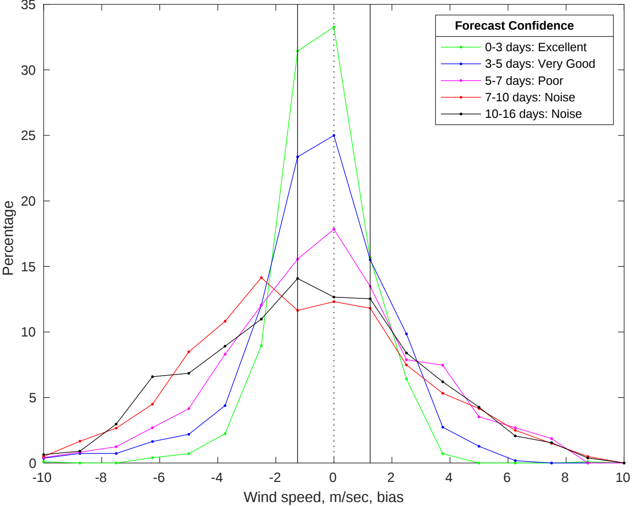
NDBC 42036 vs GFS Winds Bias Histogram: 28-Jan-2026
