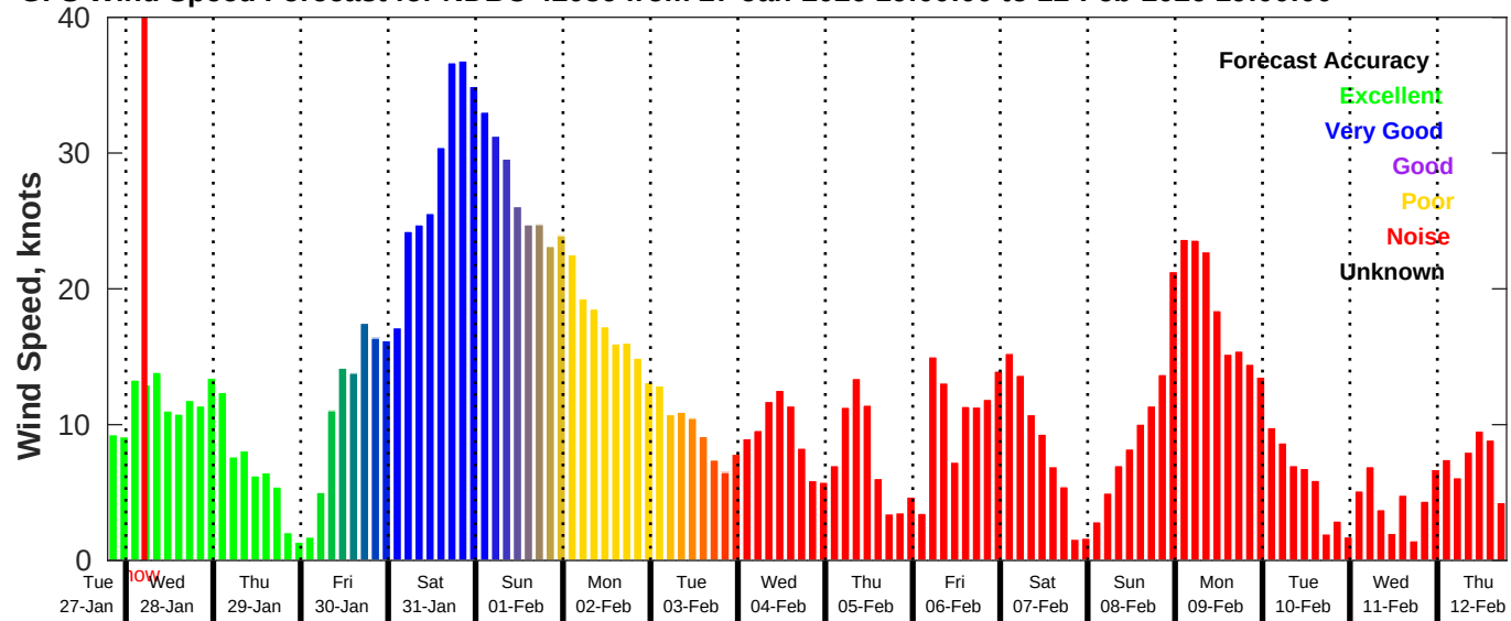
GFS Wind Speed Forecast for NDBC 42036 from 27-Jan-2026 19:00:00 to 12-Feb-2026 19:00:00
