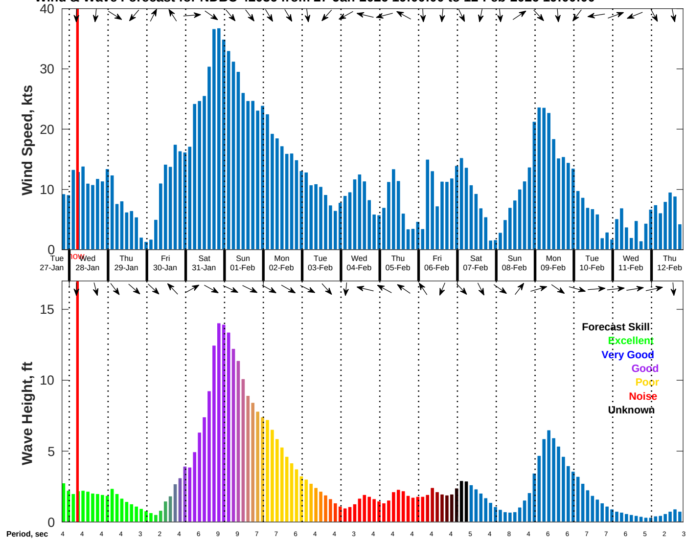
Wind & Wave Forecast for NDBC 42036 from 27-Jan-2026 19:00:00 to 12-Feb-2026 19:00:00
