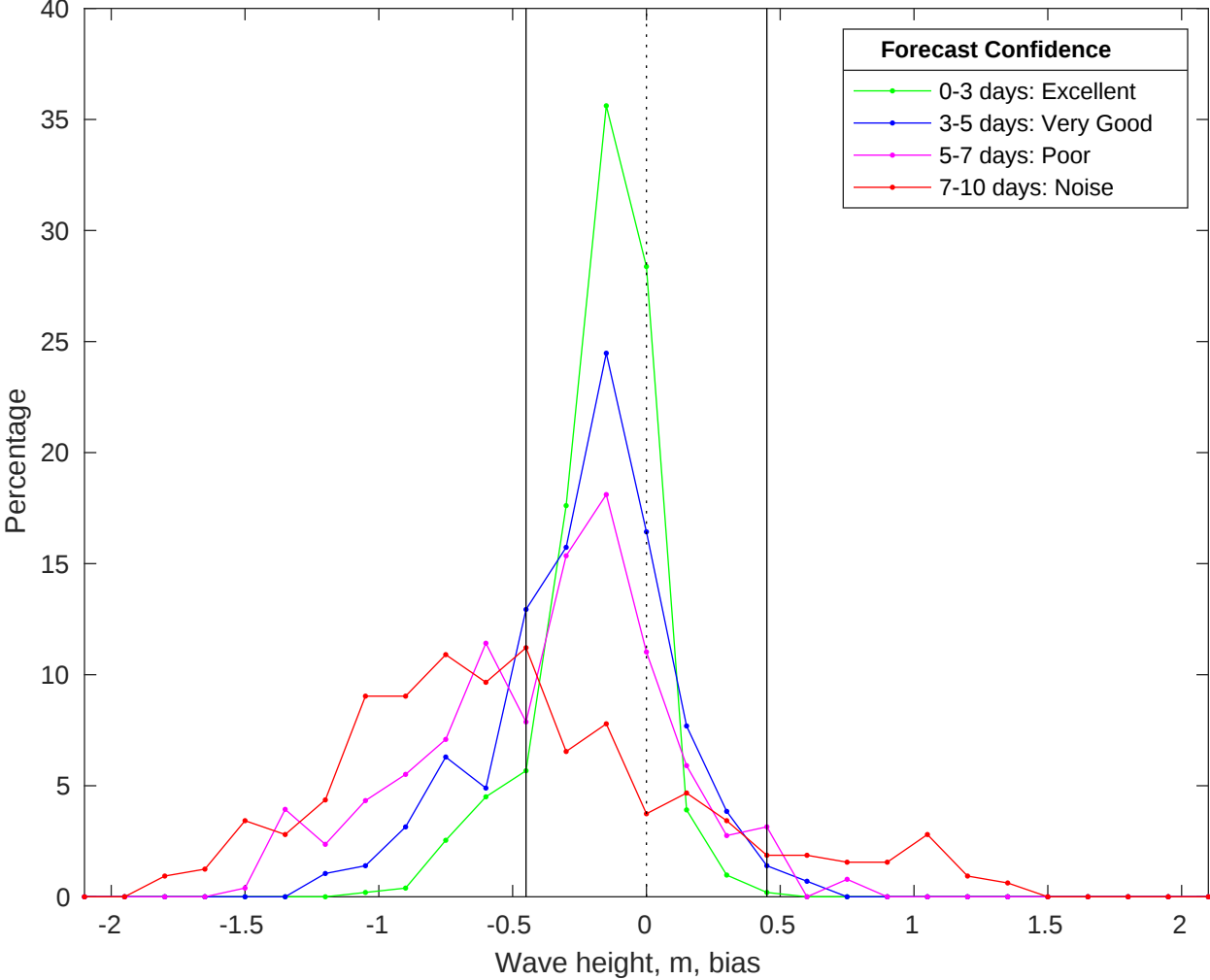
NDBC 42040 vs CMEMS Waves Bias Histogram: 28-Jan-2026
