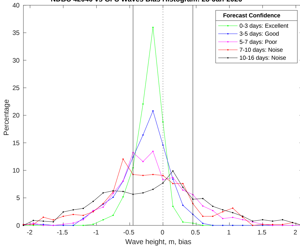
NDBC 42040 vs GFS Waves Bias Histogram: 28-Jan-2026
