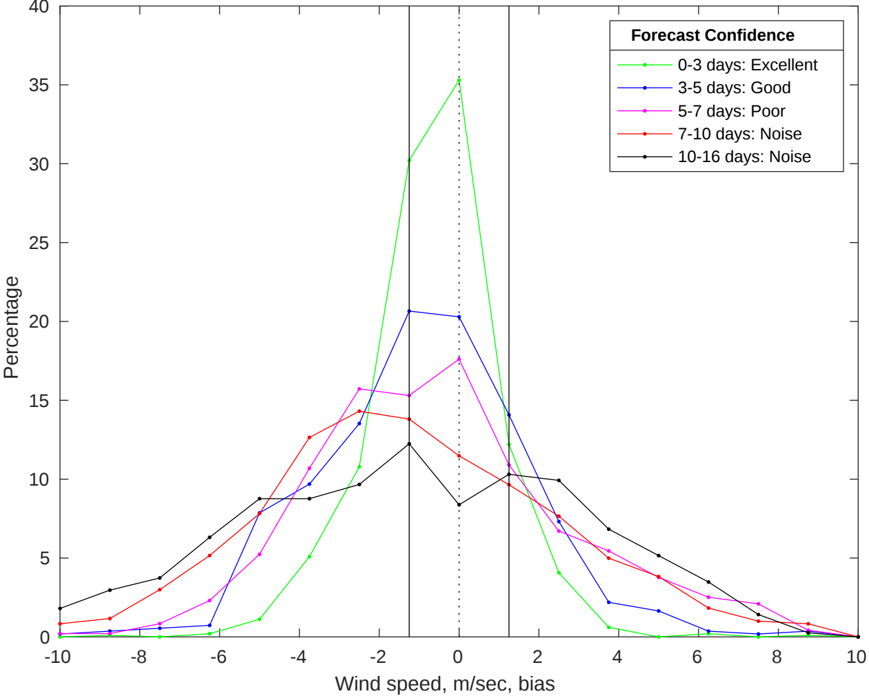
NDBC 42040 vs GFS Winds Bias Histogram: 28-Jan-2026
