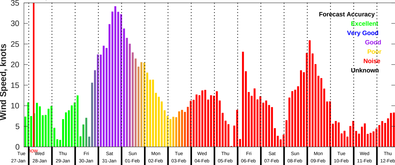
GFS Wind Speed Forecast for NDBC 42040 from 27-Jan-2026 19:00:00 to 12-Feb-2026 19:00:00
