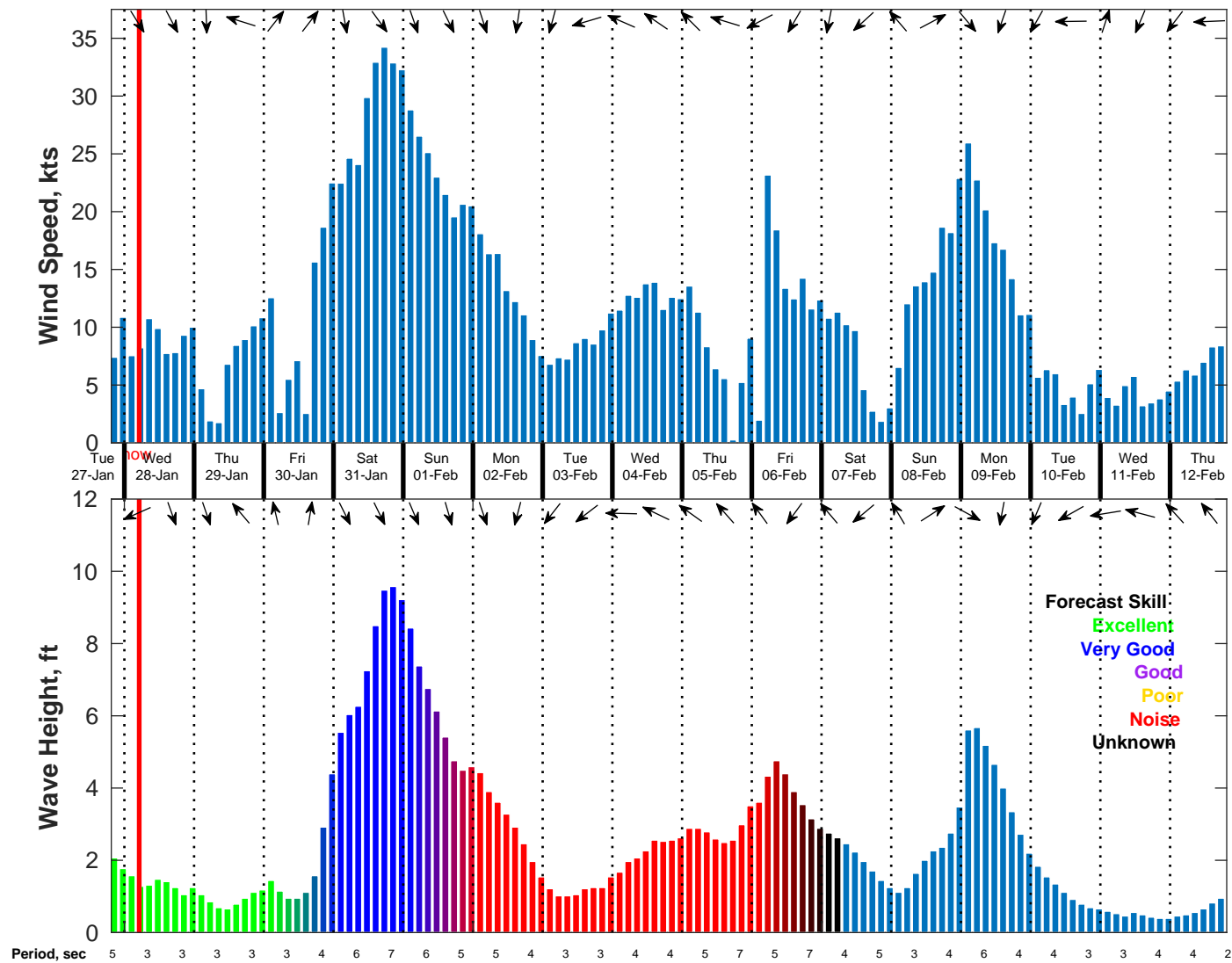
Wind & Wave Forecast for NDBC 42040 from 27-Jan-2026 19:00:00 to 12-Feb-2026 19:00:00
