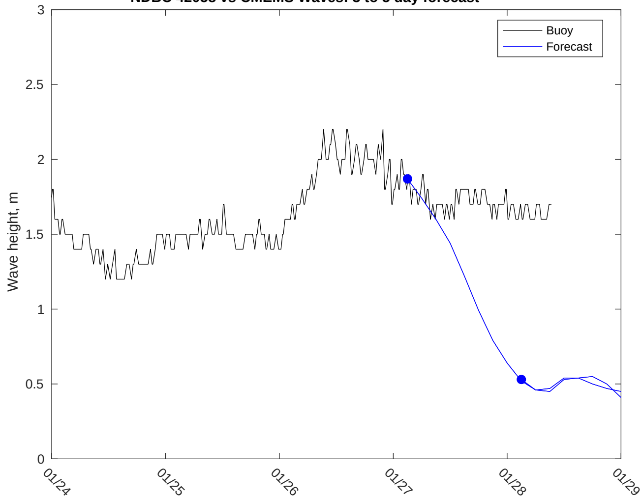
NDBC 42058 vs CMEMS Waves: 3 to 5 day forecast
