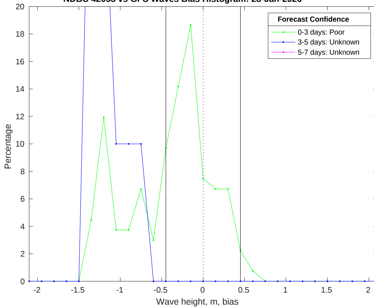
NDBC 42058 vs GFS Waves Bias Histogram: 28-Jan-2026
