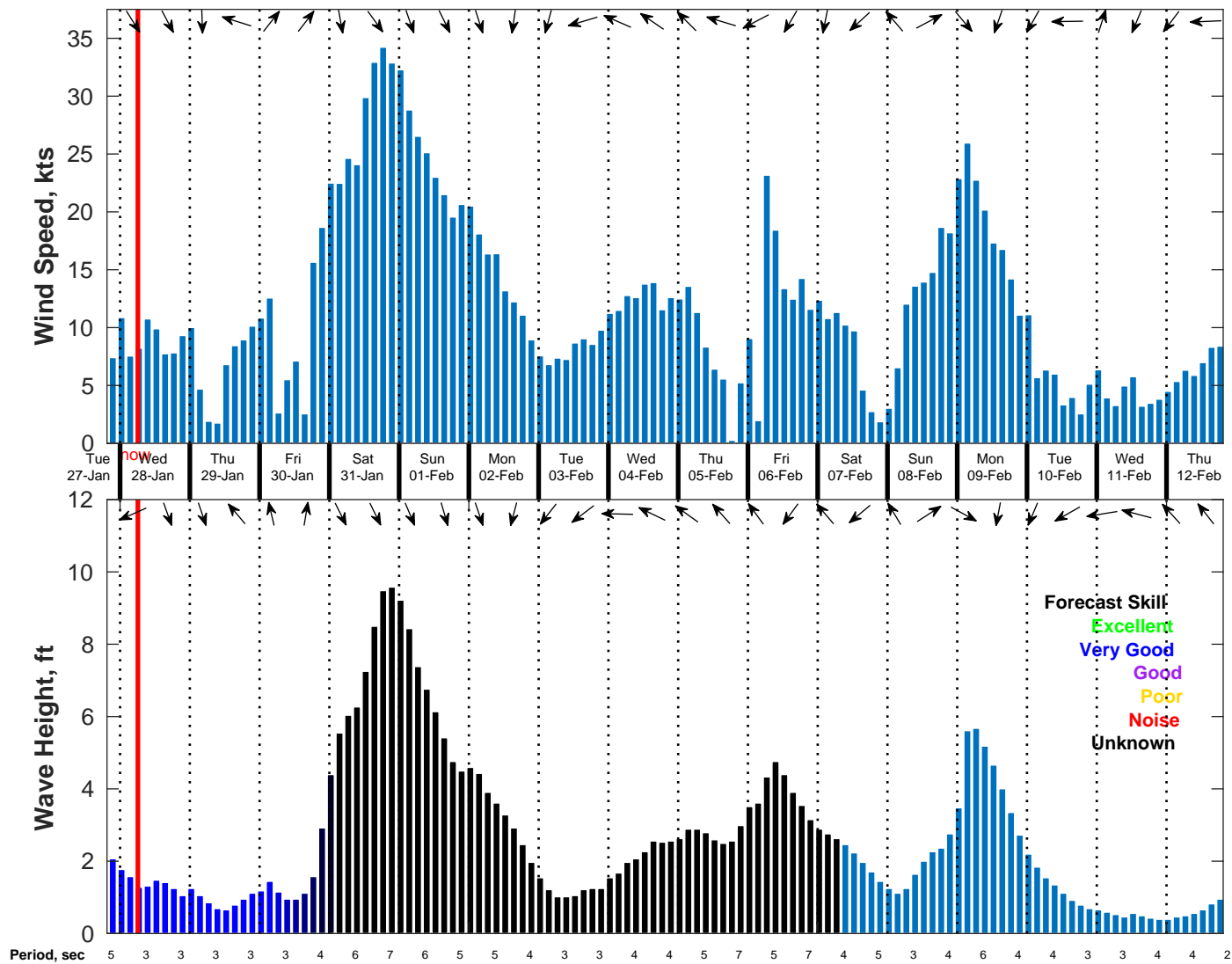
Wind & Wave Forecast for NDBC 42058 from 27-Jan-2026 20:00:00 to 12-Feb-2026 20:00:00
