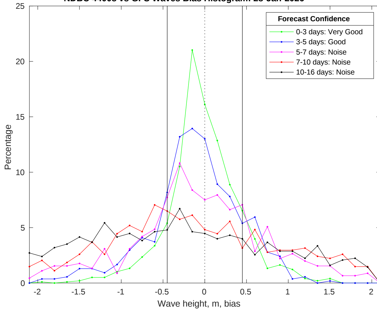
NDBC 44008 vs GFS Waves Bias Histogram: 28-Jan-2026
