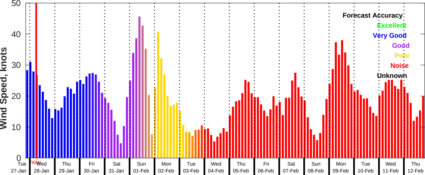
GFS Wind Speed Forecast for NDBC 44008 from 27-Jan-2026 20:00:00 to 12-Feb-2026 20:00:00
