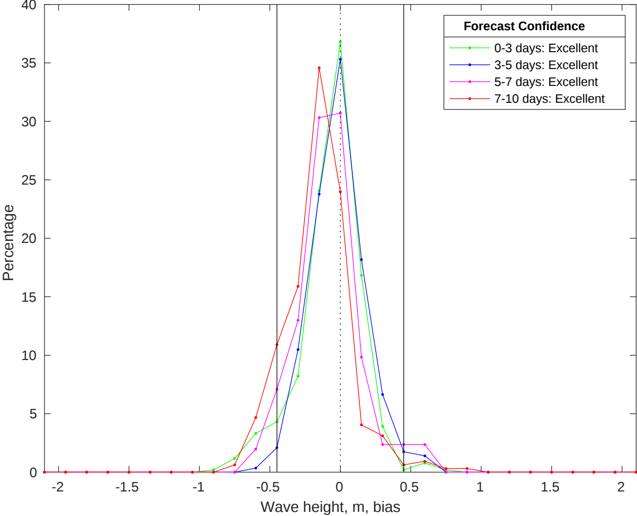
NDBC 46011 vs CMEMS Waves Bias Histogram: 28-Jan-2026
