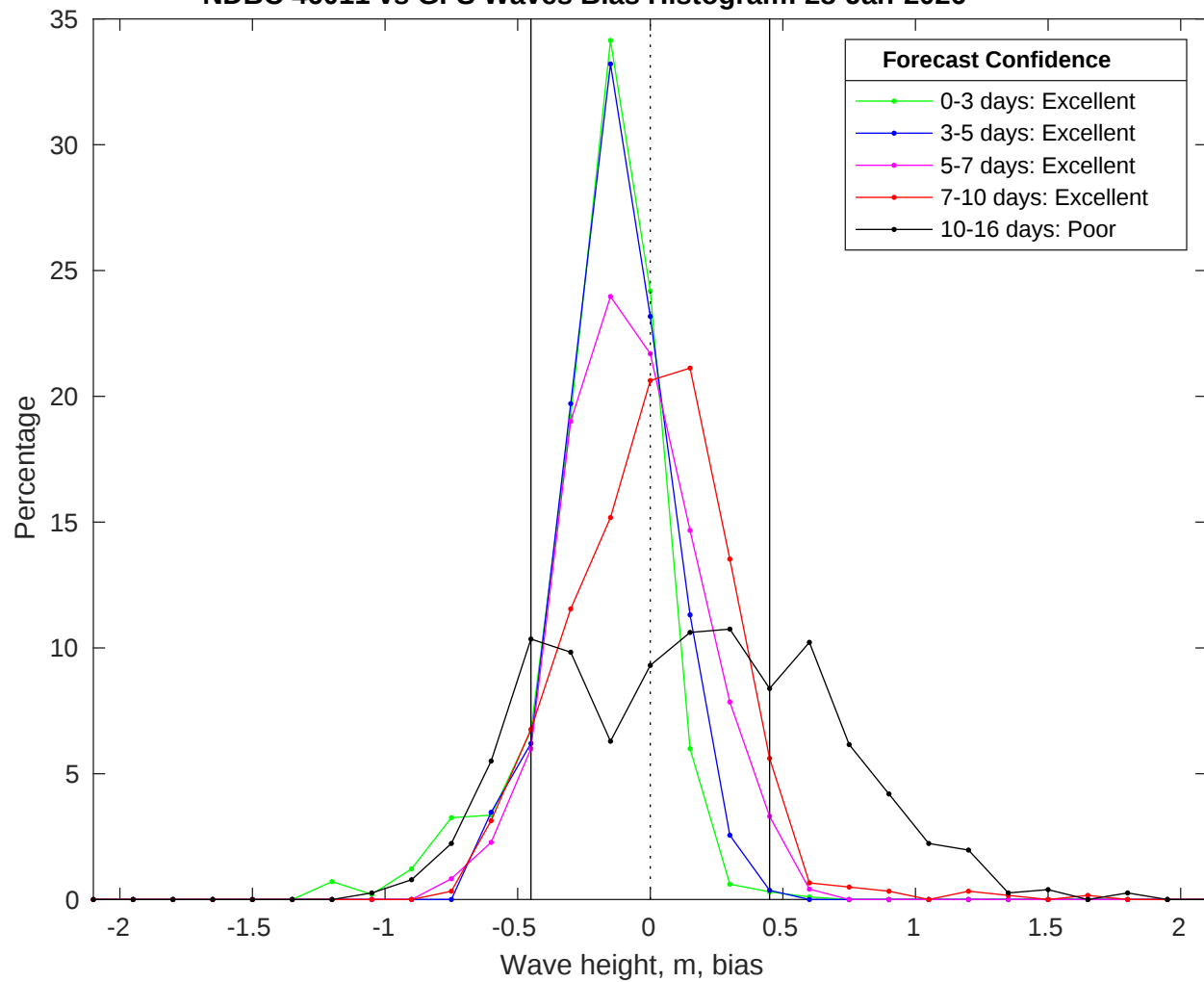
NDBC 46011 vs GFS Waves Bias Histogram: 28-Jan-2026
