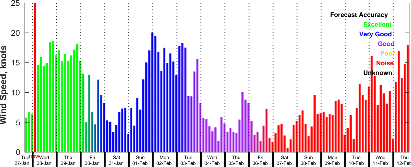
GFS Wind Speed Forecast for NDBC 46011 from 27-Jan-2026 16:00:00 to 12-Feb-2026 16:00:00
