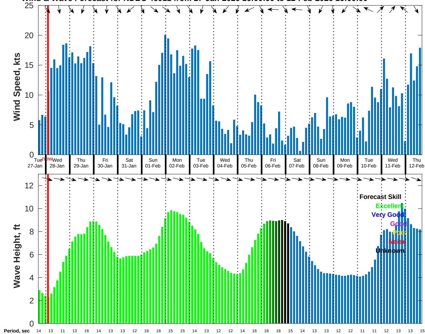
Wind & Wave Forecast for NDBC 46011 from 27-Jan-2026 16:00:00 to 12-Feb-2026 16:00:00
