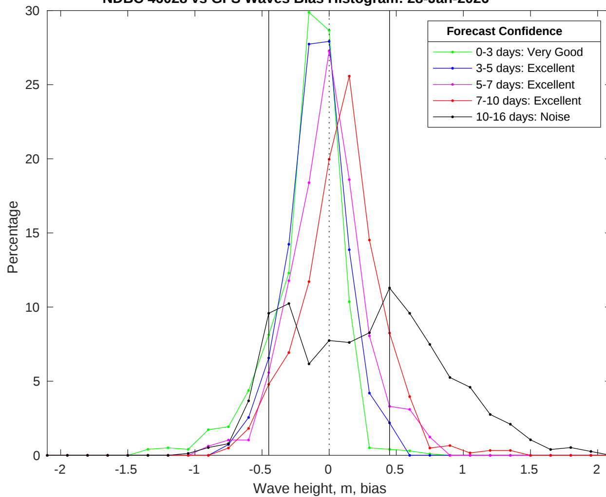
NDBC 46028 vs GFS Waves Bias Histogram: 28-Jan-2026
