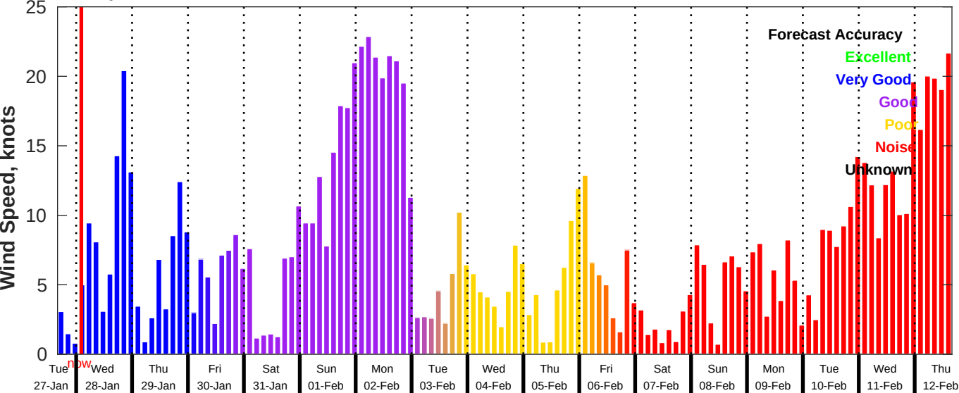
GFS Wind Speed Forecast for NDBC 46028 from 27-Jan-2026 16:00:00 to 12-Feb-2026 16:00:00
