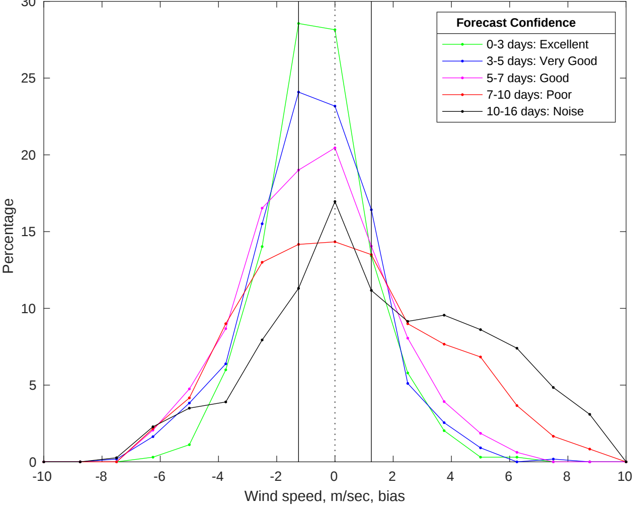
NDBC 46054 vs GFS Winds Bias Histogram: 28-Jan-2026
