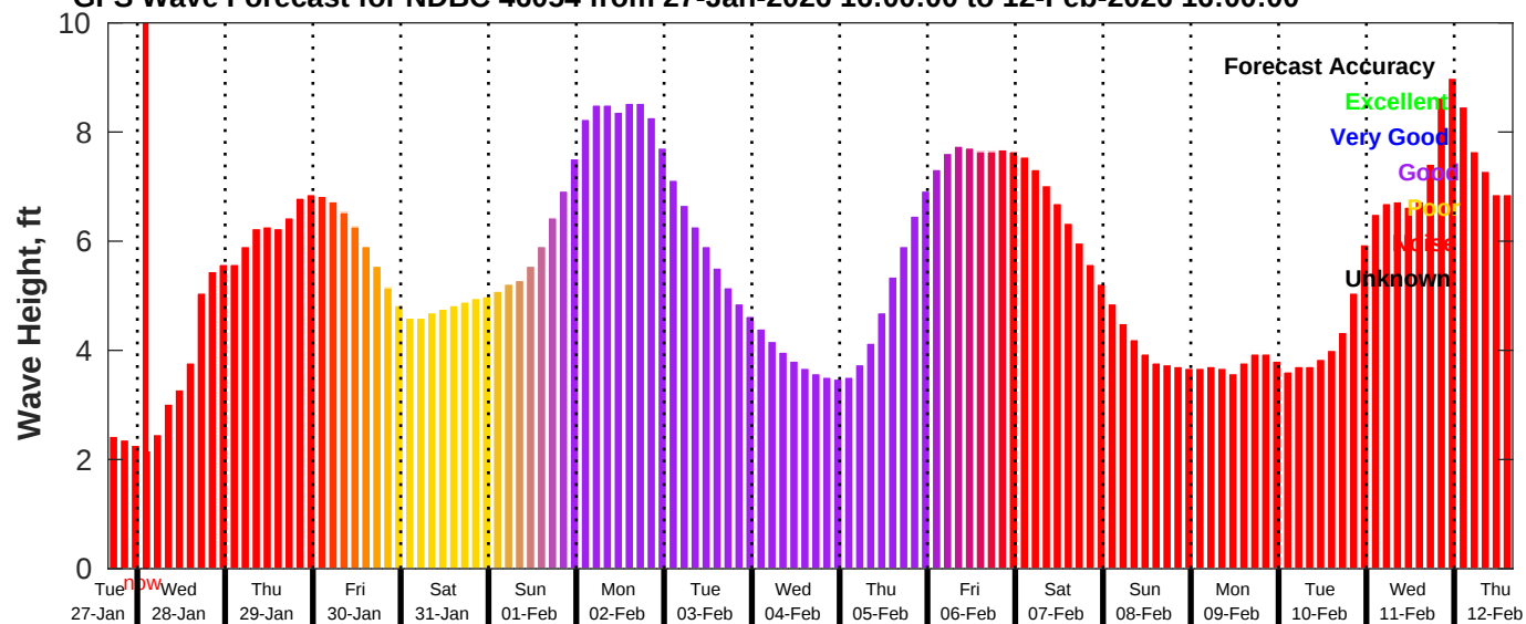
GFS Wave Forecast for NDBC 46054 from 27-Jan-2026 16:00:00 to 12-Feb-2026 16:00:00
