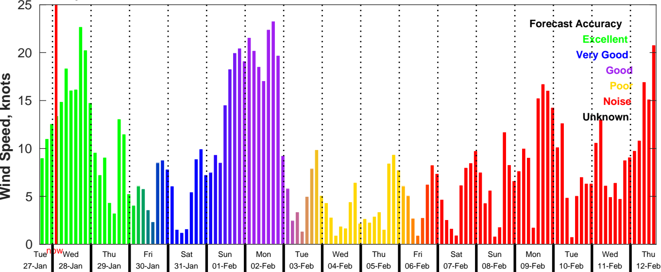
GFS Wind Speed Forecast for NDBC 46054 from 27-Jan-2026 16:00:00 to 12-Feb-2026 16:00:00
