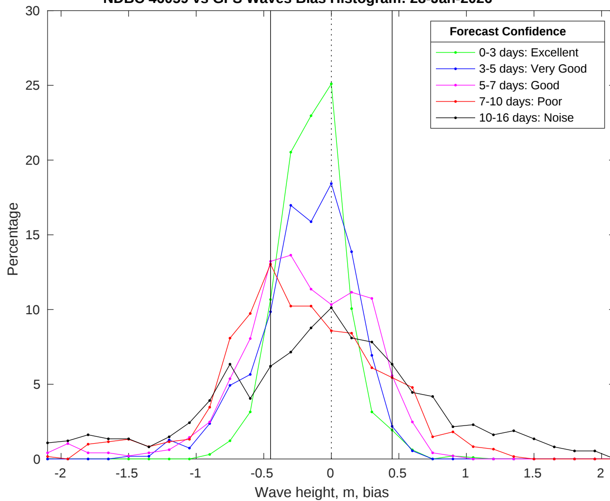
NDBC 46059 vs GFS Waves Bias Histogram: 28-Jan-2026
