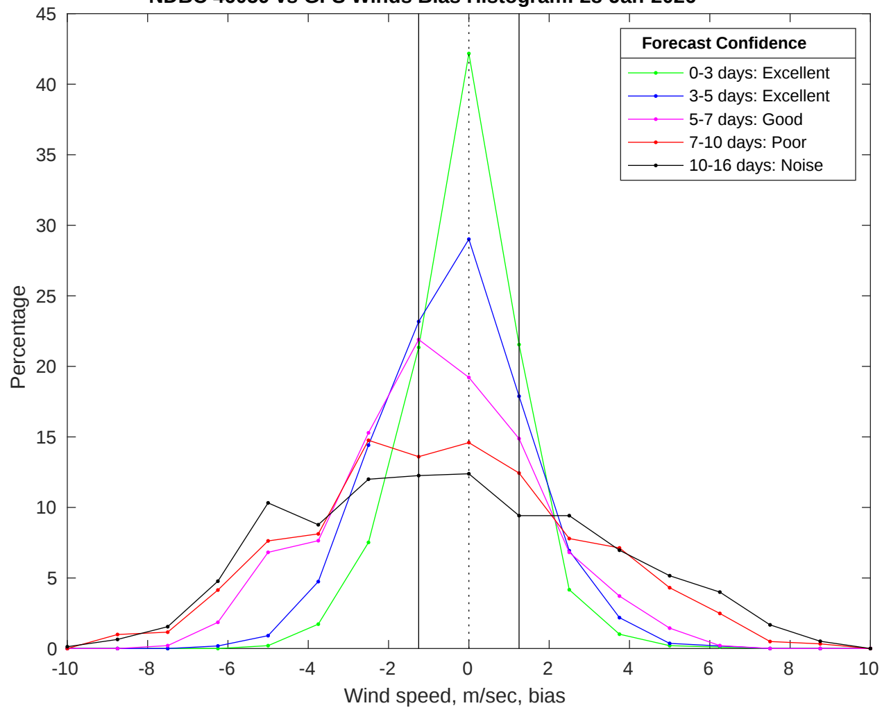
NDBC 46059 vs GFS Winds Bias Histogram: 28-Jan-2026
