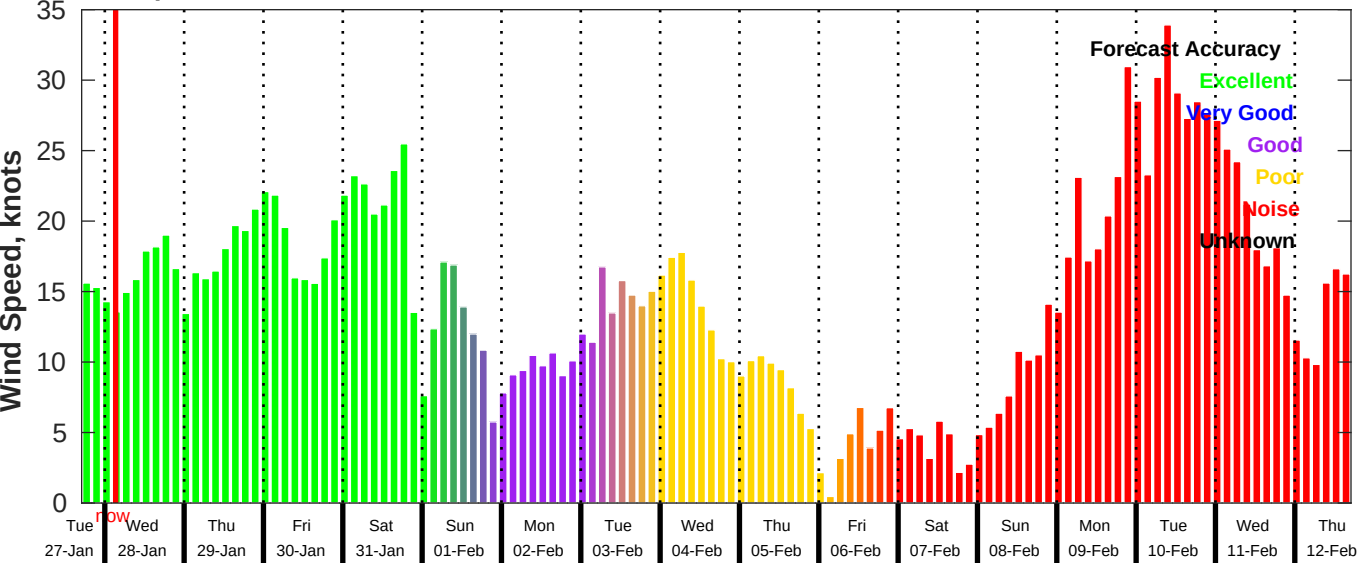
GFS Wind Speed Forecast for NDBC 46059 from 27-Jan-2026 17:00:00 to 12-Feb-2026 17:00:00
