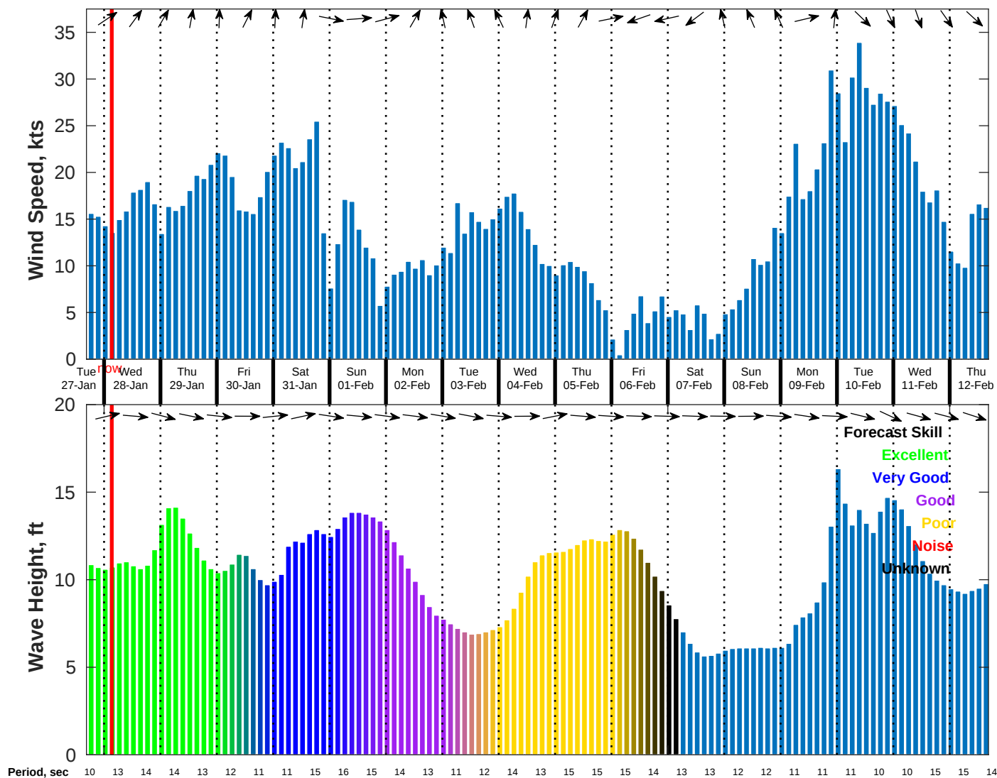
Wind & Wave Forecast for NDBC 46059 from 27-Jan-2026 17:00:00 to 12-Feb-2026 17:00:00
