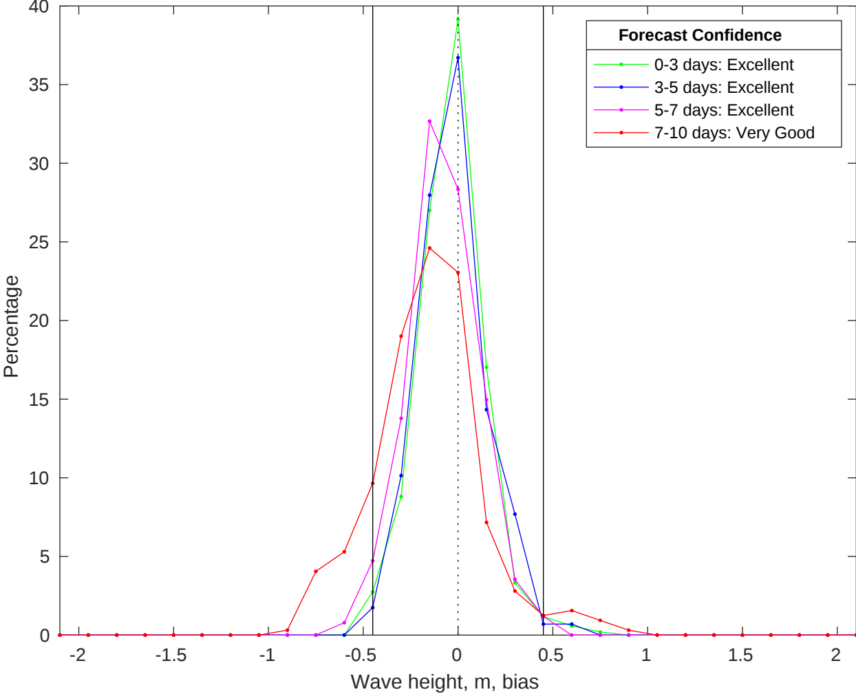
NDBC 46069 vs CMEMS Waves Bias Histogram: 28-Jan-2026
