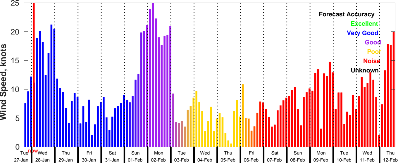
GFS Wind Speed Forecast for NDBC 46069 from 27-Jan-2026 16:00:00 to 12-Feb-2026 16:00:00
