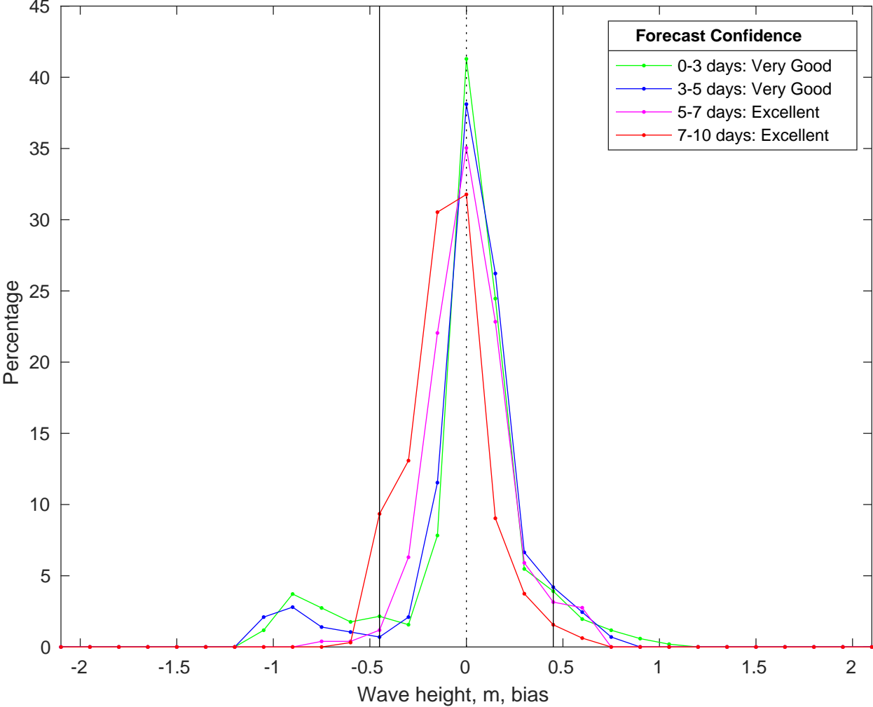
NDBC 46215 vs CMEMS Waves Bias Histogram: 28-Jan-2026
