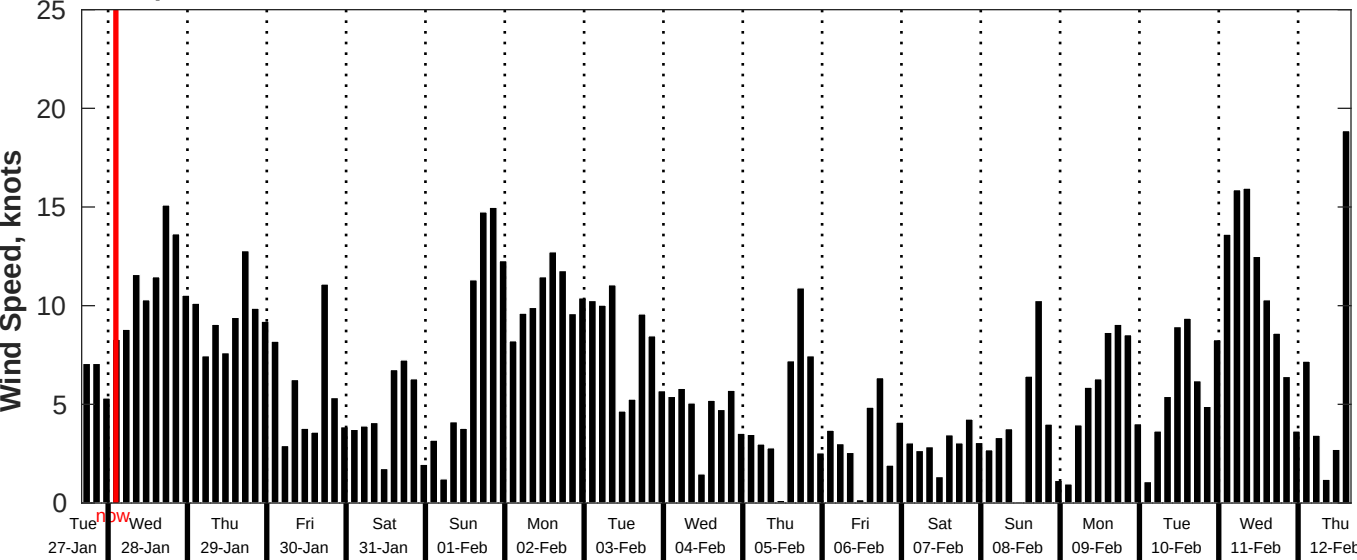
GFS Wind Speed Forecast for NDBC 46215 from 27-Jan-2026 16:00:00 to 12-Feb-2026 16:00:00
