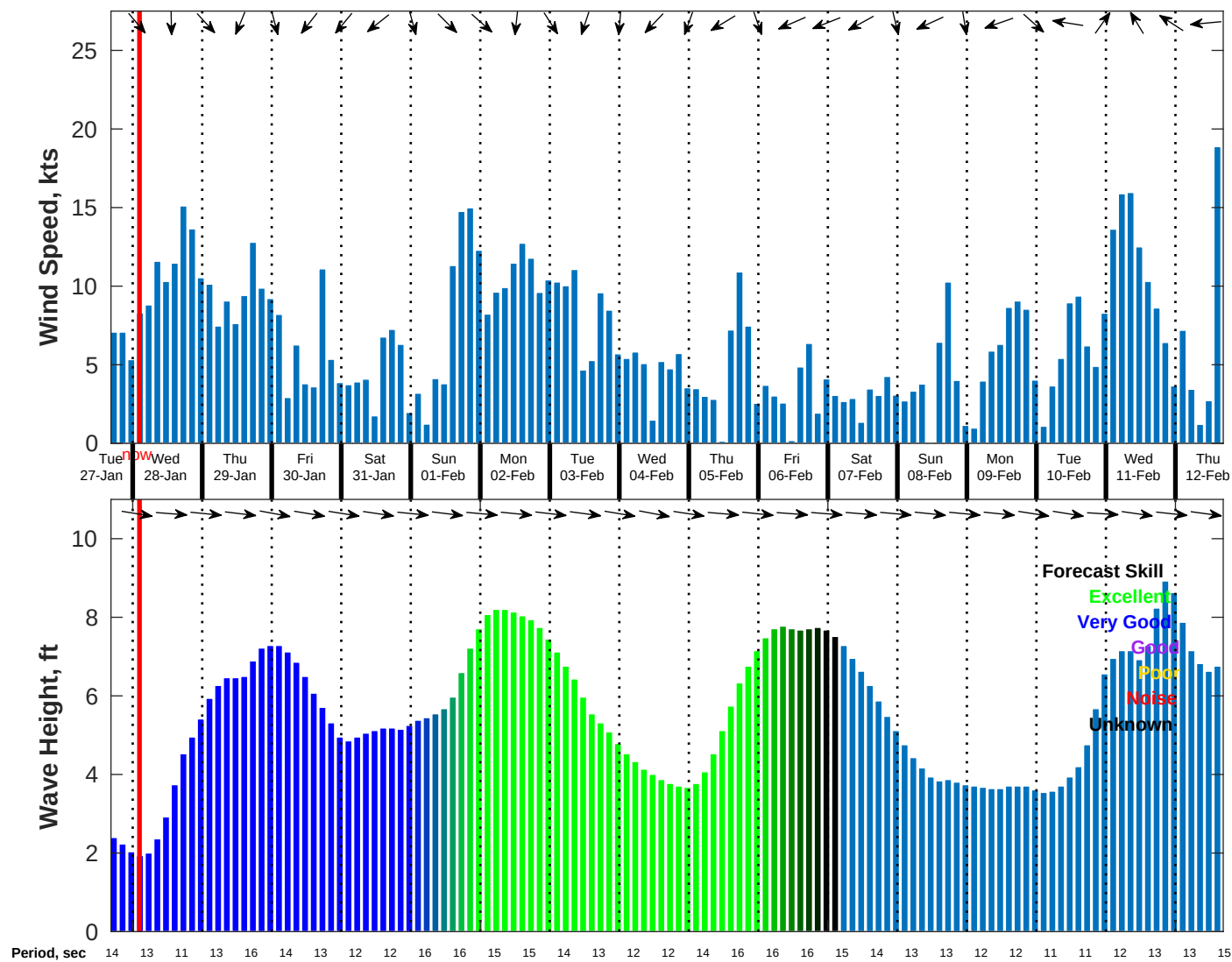
Wind & Wave Forecast for NDBC 46215 from 27-Jan-2026 16:00:00 to 12-Feb-2026 16:00:00
