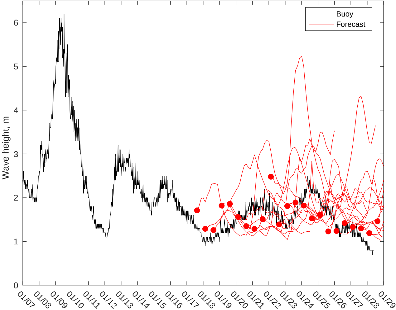
NDBC 46259 vs GFS Waves: 10 to 16 day forecast
