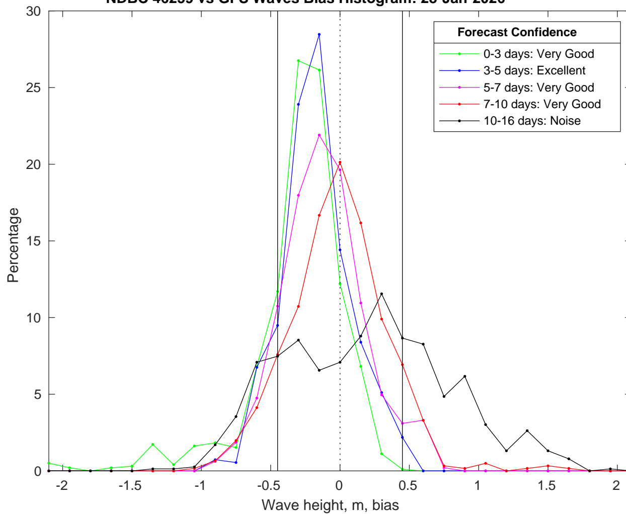
NDBC 46259 vs GFS Waves Bias Histogram: 28-Jan-2026
