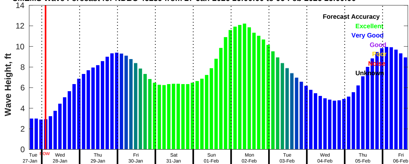
CMEMS Wave Forecast for NDBC 46259 from 27-Jan-2026 16:00:00 to 06-Feb-2026 16:00:00
