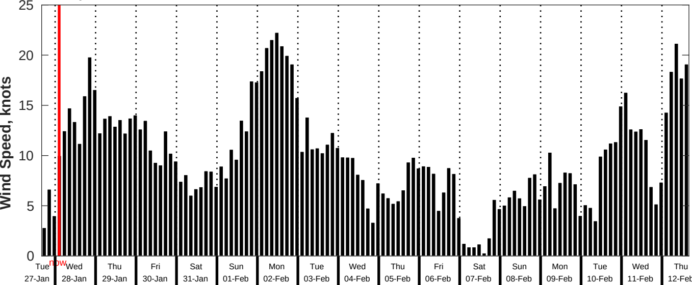
GFS Wind Speed Forecast for NDBC 46259 from 27-Jan-2026 16:00:00 to 12-Feb-2026 16:00:00
