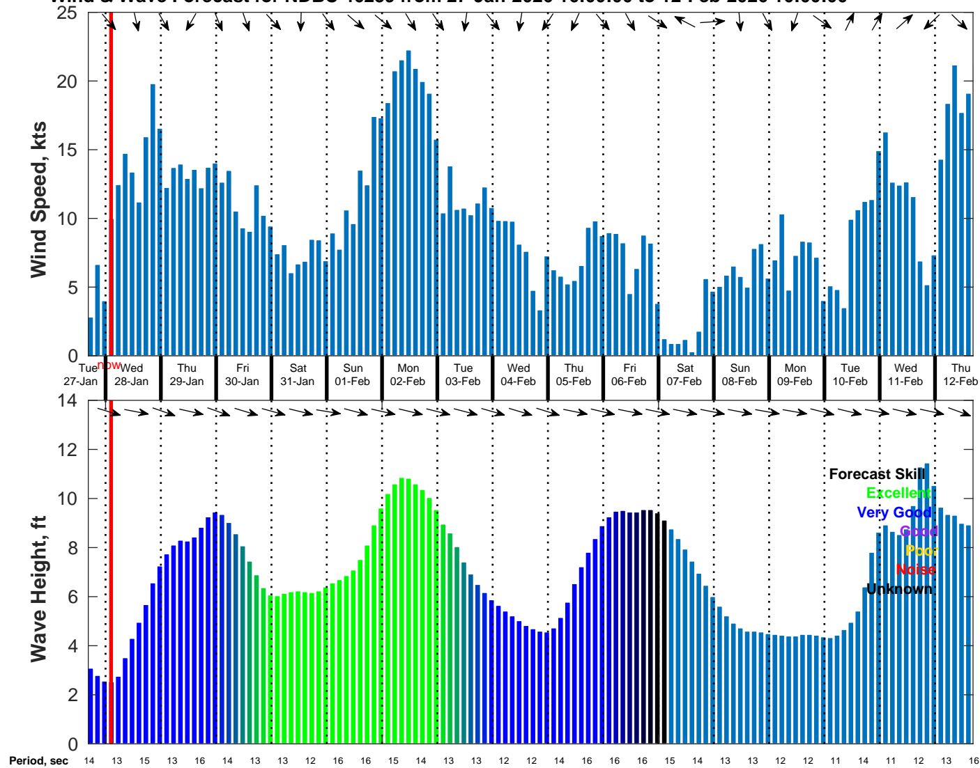
Wind & Wave Forecast for NDBC 46259 from 27-Jan-2026 16:00:00 to 12-Feb-2026 16:00:00
