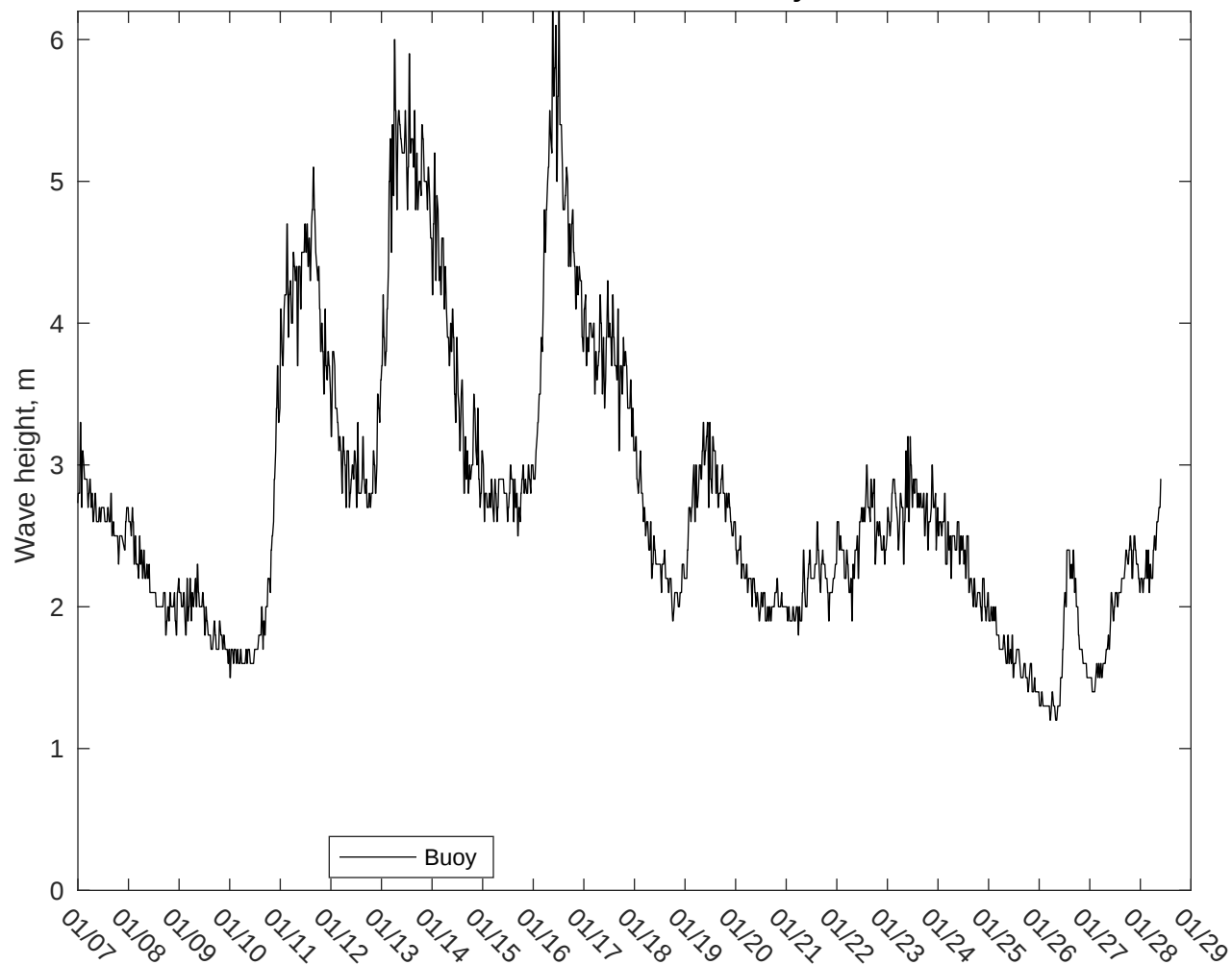
NDBC 51000 vs CMEMS Waves: 10 to 16 day forecast
