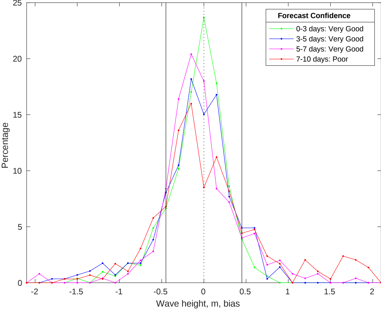
NDBC 51000 vs CMEMS Waves Bias Histogram: 28-Jan-2026
