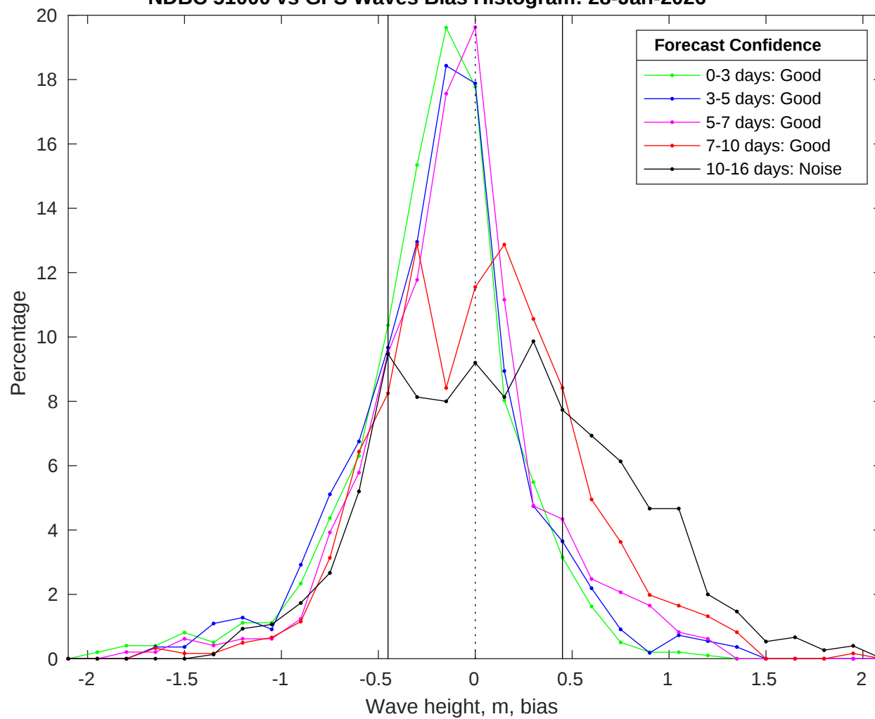
NDBC 51000 vs GFS Waves Bias Histogram: 28-Jan-2026
