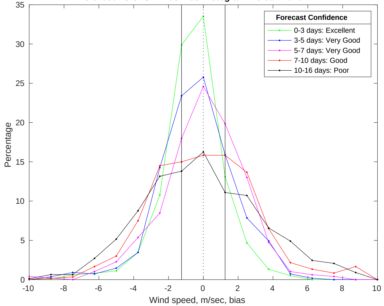
NDBC 51000 vs GFS Winds Bias Histogram: 28-Jan-2026
