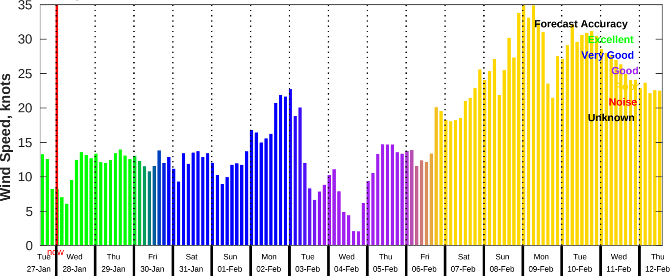
GFS Wind Speed Forecast for NDBC 51000 from 27-Jan-2026 14:00:00 to 12-Feb-2026 14:00:00
