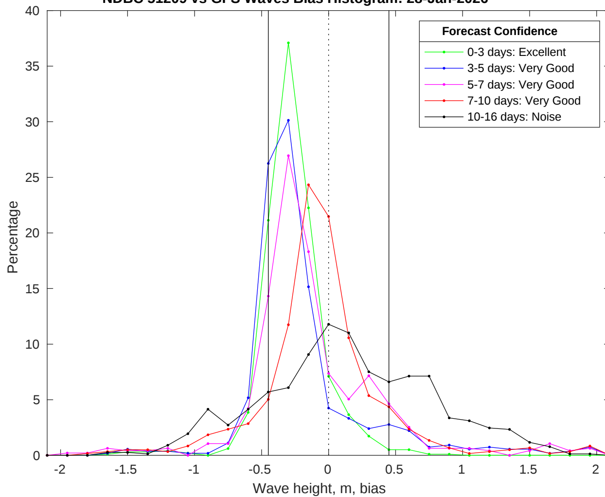
NDBC 51209 vs GFS Waves Bias Histogram: 28-Jan-2026
